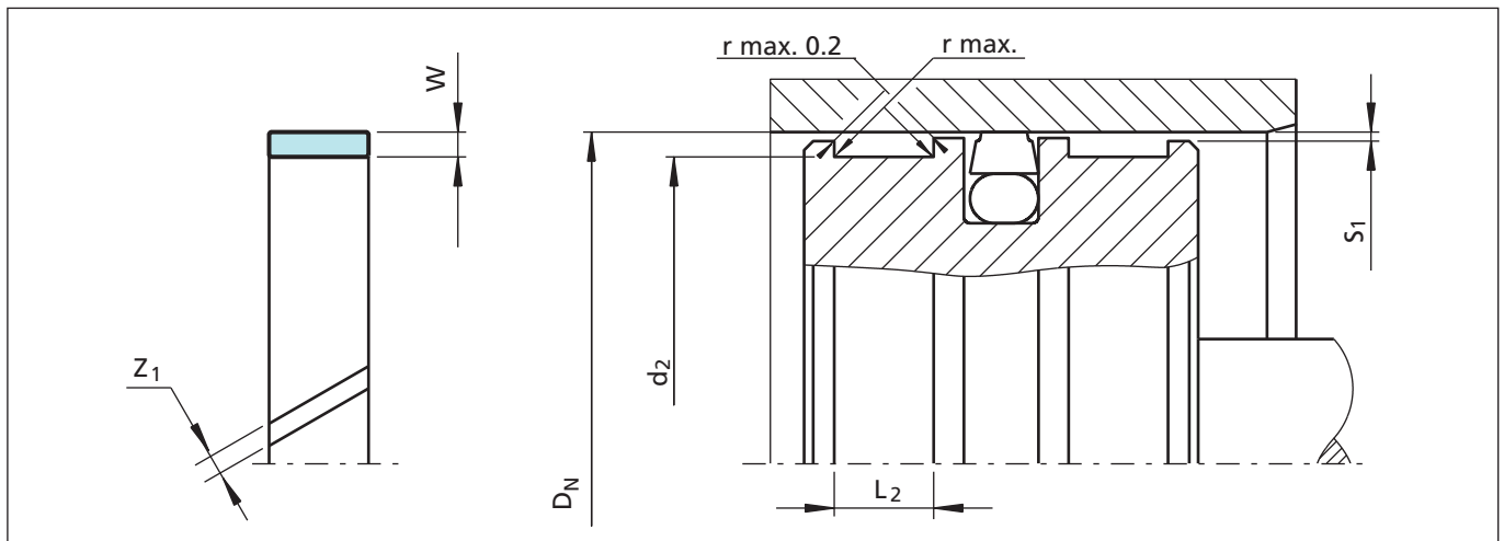
Figure 11 Installation drawing
