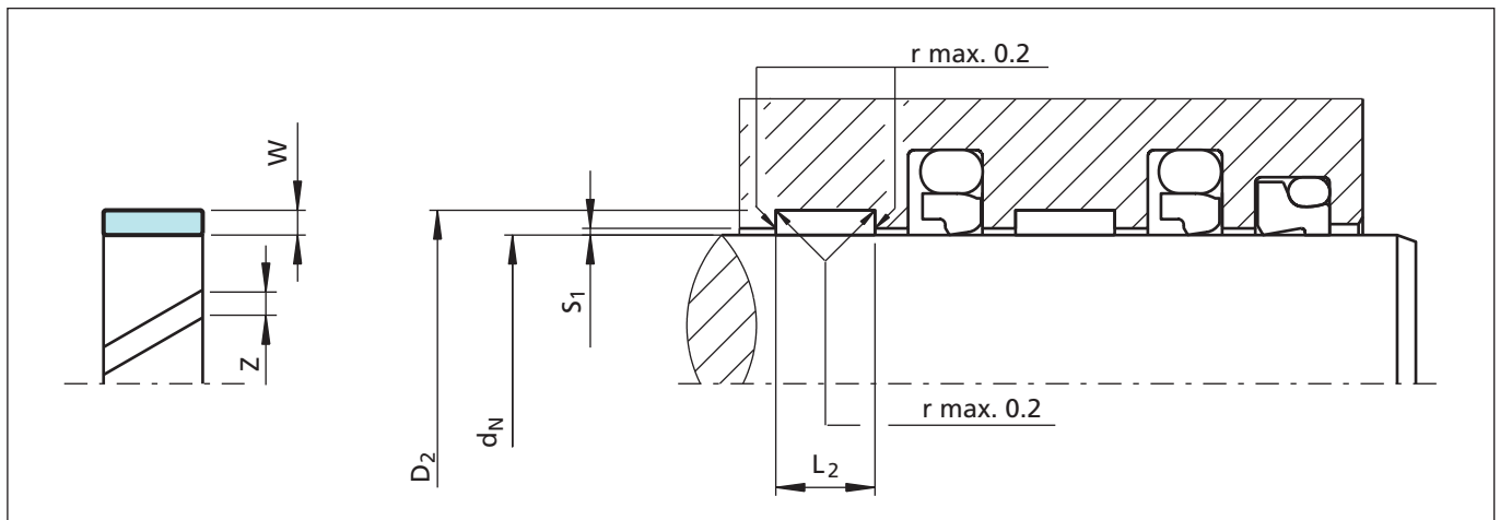
Figure 10 Installation drawing
